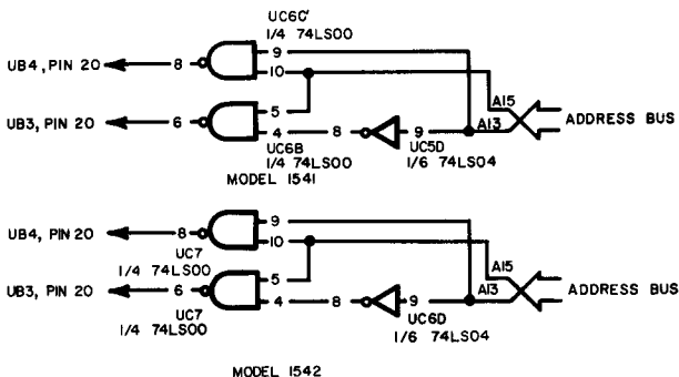
Fig. 7-45. ROM address decoder changes, Model 1542.
